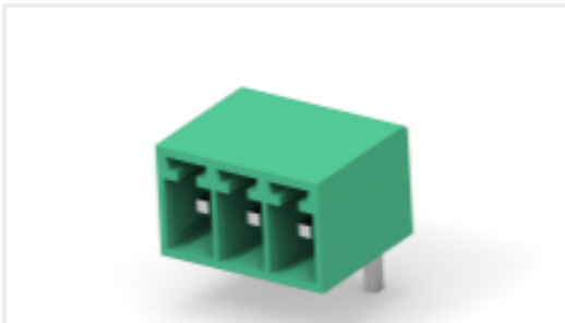
TE 产品编号2350514-3 3POS TB HDR 90 DEG, PITCH 3.5 & TL 3.5mm
