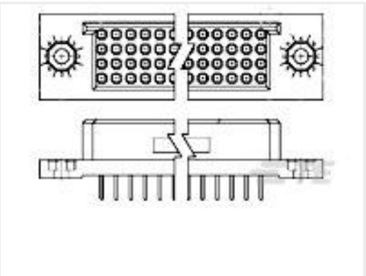
TE 产品编号533492-1 BOX II 4 ROW RECP ASSY 160 POS
