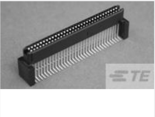
TE 产品编号2-5120524-2 1FHR,84,30A/S,R,N,S14,15
