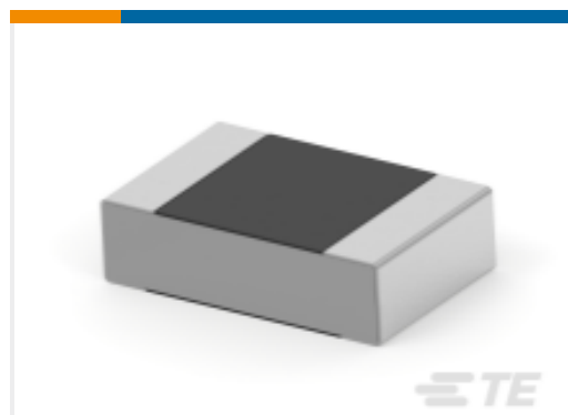
TE 产品编号6-2176238-8 CPF A 0805 200K 0.1% 25PPM 5K RL
