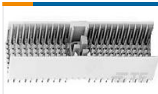
TE 产品编号6645141-1 2MM H.M. 8 + 2 ROW TYPE "F" PI
