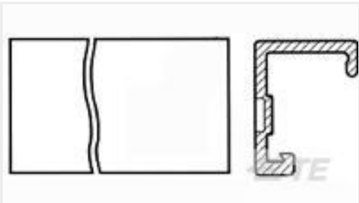
TE 产品编号640551-6 06P MTA156 COVER
