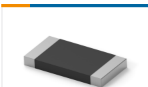
TE 产品编号4-2176422-7 TLRP 2512 3.0W R003 1% 50PPM 4K RL
