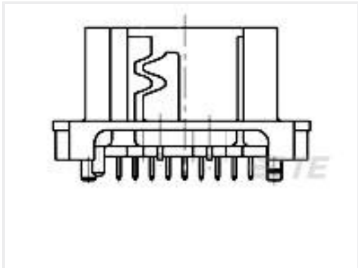
TE 产品编号967618-2 18pos MQS .63 header 180deg
