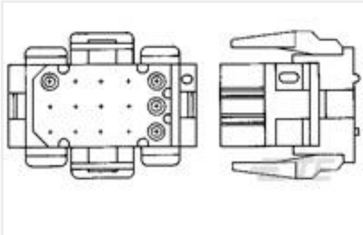
TE 产品编号1-640521-0 09P MR II PLUG HSG V0
