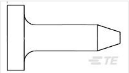
TE 产品编号206509-1 SIZE 20 KEYING PLUG
