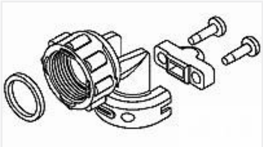
TE 产品编号796380-2 R/A STRN RELIEF KIT,SZ 13,CPC
