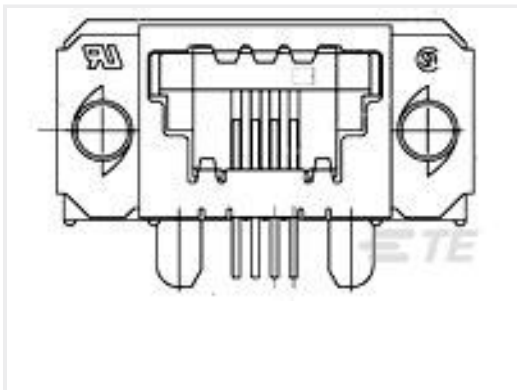
TE 产品编号4-1761206-1 4 SDL SE RCPT ASSY PART SHELD
