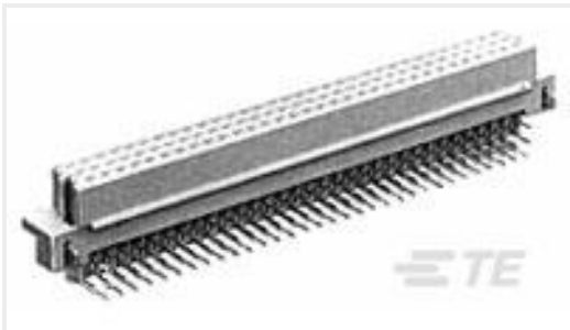
TE 产品编号5650874-4 ASSY,RECEPTACLE,EUROCARD,TYPE
