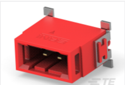
TE 产品编号294648-E SRCP 2,54 2 M 1 SMD 137 E1 168 * GU-H *
