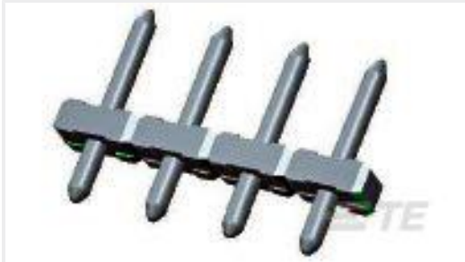
TE 产品编号282832-2 TERMI-BLOK PIN HEAD 180 2P. 5
