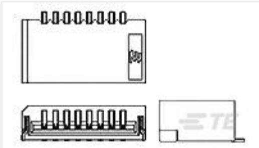
TE 产品编号CAT-104MTA-PVUNH PCB Header: Polyester, Vertical, Unshrouded, No Mating Alignment
