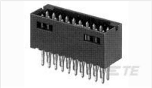
TE 产品编号2-6450540-5 MBXL VERT RCPT 2P+24S+2P
