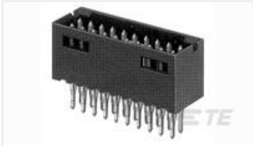
TE 产品编号2170901-1 HM-EZD,ASSEMBLY,VT,4PAIR,10COL
