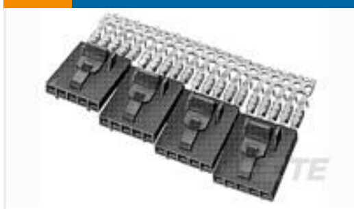
TE 产品编号 5-103960-5 4X6 MTE RCPT SR LATCH .100CL
