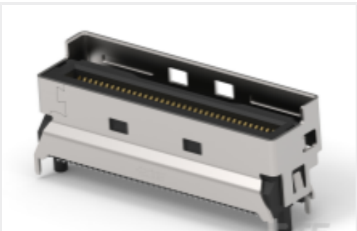
TE 产品编号2379397-6 MCIO INTERGRATED CONN, V/T,8X, SMT TYPE
