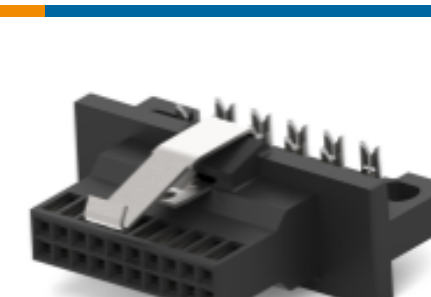
TE 产品编号 5-104892-8 80 50/50 GRID RCPT W/LTCH LF
