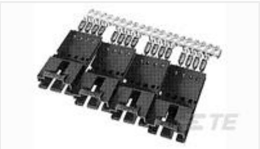
TE 产品编号5-103945-1 8X2 MTE SHRD PIN SR LATCH .100
