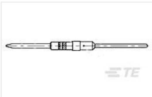
TE 产品编号1-448139-1 CNCT, SZ 16 PSTD PIN
