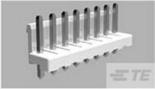
TE 产品编号5-1123723-5 3.96 EP HDR ASSY 5P(BLACK)
