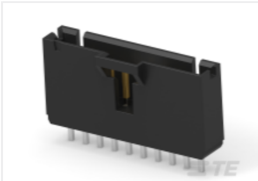
TE 产品编号 5-104362-9 10 MTE HDR SRST LATCH W/HLDWN
