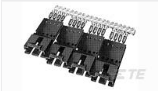
TE 产品编号5-103949-9 2X10 MTE SHR PIN SR LTCH .100
