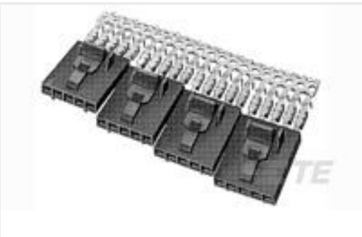
TE 产品编号5-103957-4 4X5 MTE RCPT SR LATCH .100CL
