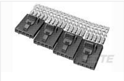
TE 产品编号5-103957-6 2X7 MTE RCPT SR LATCH .100CL
