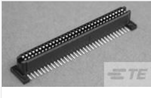
TE 产品编号5146893-2 1FHR,84,30A/S,S,C,S08,09,10
