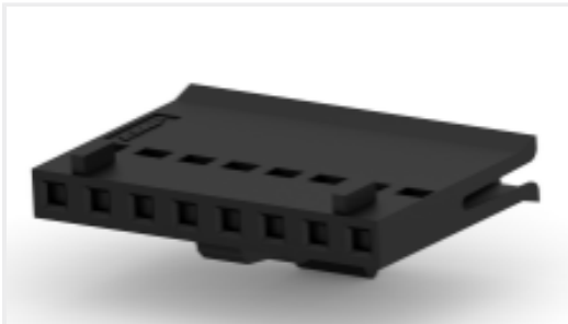
TE 产品编号 487526-7 008 HOUSING FFC RCPT 100CL SR
