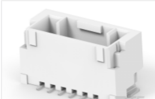
TE 产品编号2360540-6 SGI 1.25 HDR, 6P, VT, Key A, Natural
