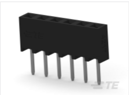
TE 产品编号2314868-6 6P,2MM,BB,REC,SRVT,2.0,0.1AU,TB,W/CP
