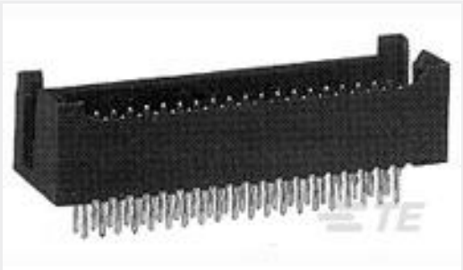
TE 产品编号6-102567-2 40 MODII 2PC HDR DR SHRD .100,
