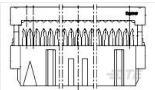
TE 产品编号2-215911-0 20 WAY BLACK MK II RECP
