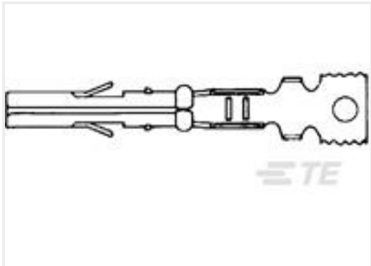
TE 产品编号641300-1 MR RECPT PTPHBZ LP 26-18
