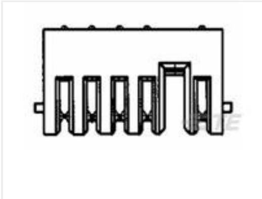
TE 产品编号1473971-2 REC ASS'Y V TYPE FOR 2.5MM PIT
