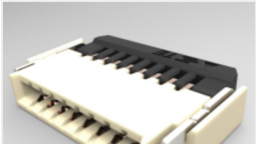
TE 产品编号1-2328702-0 10PIN 0.5MMP FPC CONN, BACK FLIP LOCK
