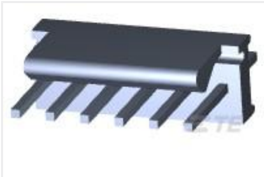
TE 产品编号3-641126-6 06P MTA100 HDR ASY FL/STR LF
