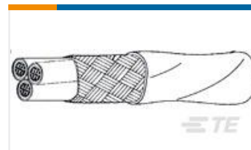
TE 产品编号880559-000 44AM1131-24-MST3-9CS2275
