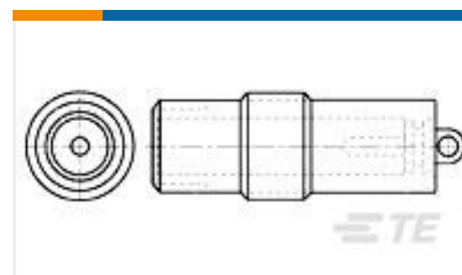
TE 产品编号448464-1 LGH 1/2, RCPT, MOD, W/3/8-24 UNF
