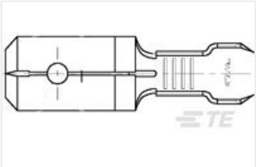
TE 产品编号626377-1 TERMINAL FASTON .250 TAB 22-18 AWG BR
