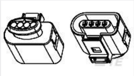
TE 产品编号1599632-1 HOUSING ASSY 4 POSN 2,8 mm REC JPT
