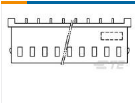
TE 产品编号1470222-2 HPI 2.5MM EMIX HOUSING 2P
