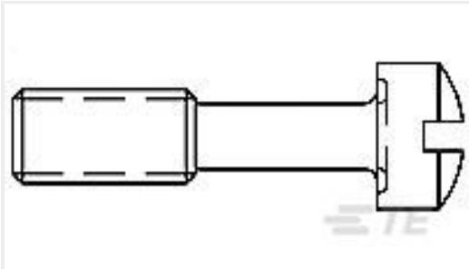
TE 产品编号5206052-3 SCREW,SPECIAL,ZN
