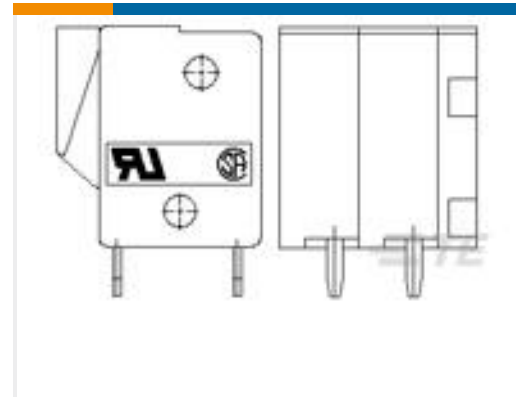
TE 产品编号1-1776260-0 10P Spring TB, 180deg, VT,5.08mm, Green
