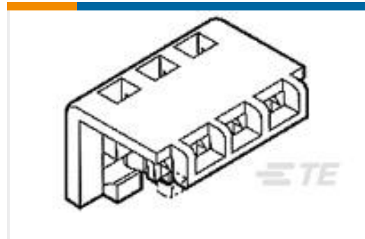
TE 产品编号1-643067-0 10P MTA156 MOLDED COVER
