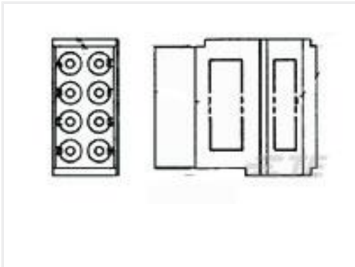
TE 产品编号1-592620-1 TERM JCT,F/B,SZ 16,07 BUSSING
