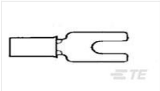
TE 产品编号41495 SPADE .190(4.82 MM)12-10 AWG TPBR
