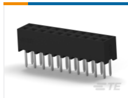
TE 产品编号2-2314826-0 20P, 2MM, B-B, REC, DRVT, 2.7, 0.76AU, TB, W/CAP
