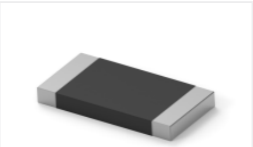
TE 产品编号3-2176422-7 TLRP 2512 3.0W R075 1% 25PPM 4K RL
