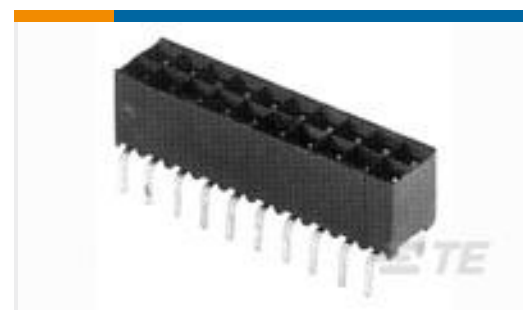
TE 零件编号 6-969982-8 AMPMODU II Action Pin Header, dual row
