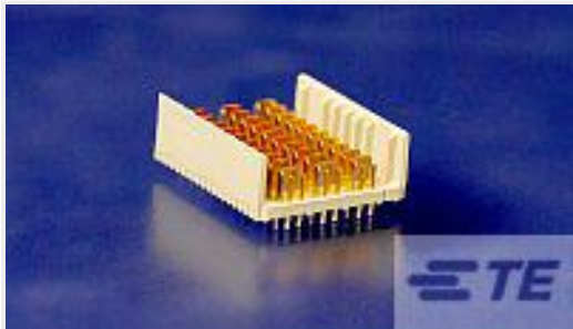
TE 产品编号6469085-1 HMZD 3PAIR, HDR ASSY, 25MM MOD
