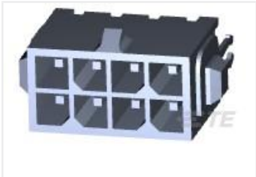
TE 产品编号3-794681-8 08P MICRO MNL ASSY,VRT,THRU,LF
