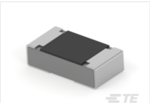
TE 产品编号4-2176480-4 RA73F 1J 1K54 0.1% 5K RL
