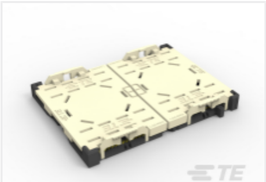
TE 产品编号1-2324271-1 RIGHT SEGMENT LGA4189-4 SOCKETP4 FOR ODM
